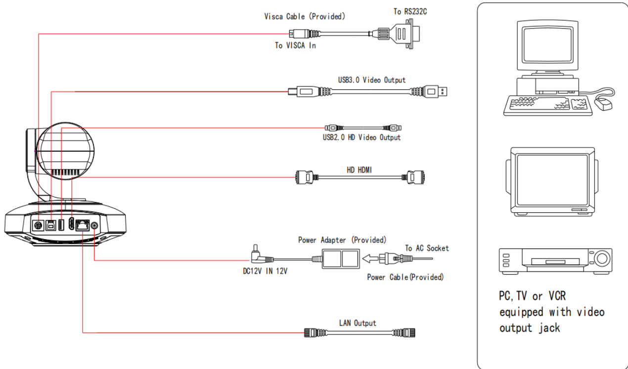
Figure1-5 Interface Diagram
