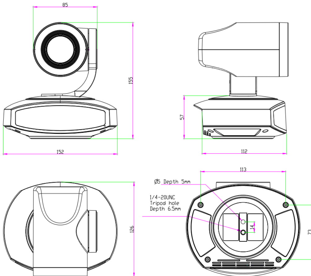
Figure1-4 Product Dimension
