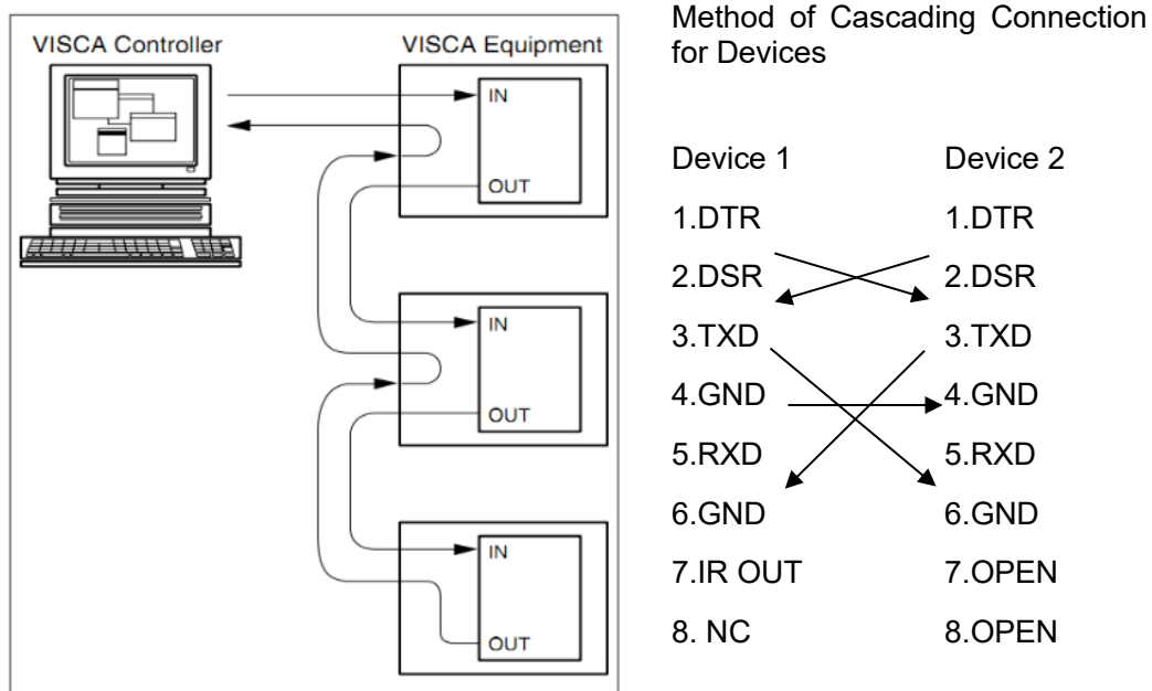
Figure 2-4 VISCA Schematic Diagram of Networking Configuration
